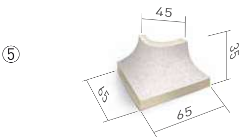
Outer angle corner Esquina cantonera exterior MDCA AE000 6.5x6.5
