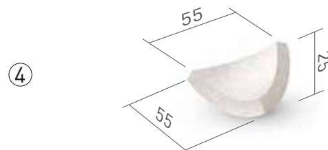
Scotch inner corner Escocia cantonera interior MDCA EI000 5.5x5.5
