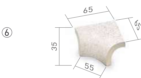
Inner angle corner Esquina cantonera interior MDCA AI000 6.5x6.5
